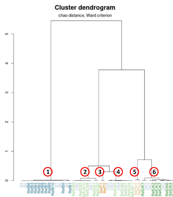
Figure 6. Final cluster tree. 1. Brazil clade; 2. US clade 1; 3. Thailand clade 3; 4. US clade 2; 5. Turkey clade and 6. UK clade.
