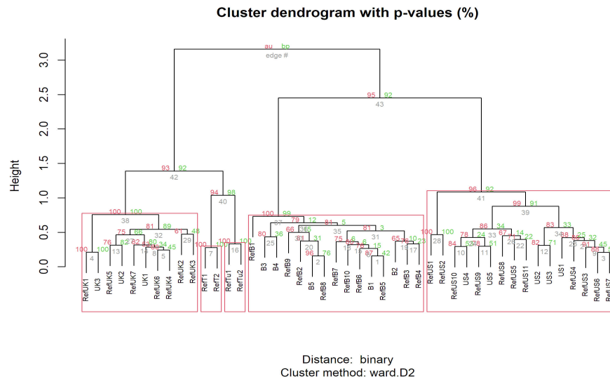
Figure 7. Cluster dendrogram after assessment using pvclust.
