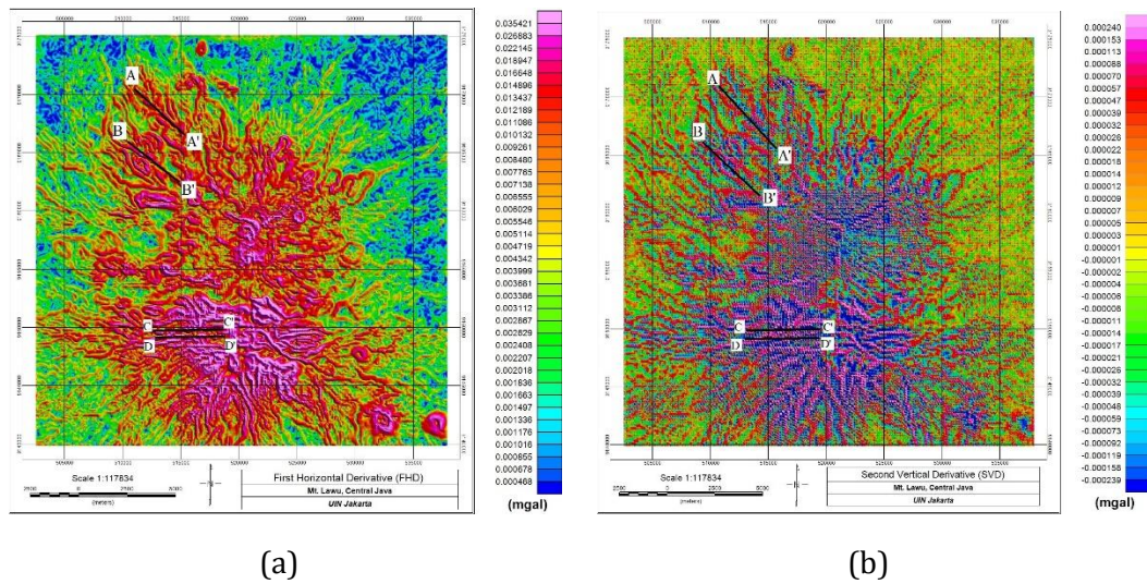
Figure 6. (a) First Horizontal Derivative (FHD) Map, (b) Second Vertical Derivative (SVD) Map
