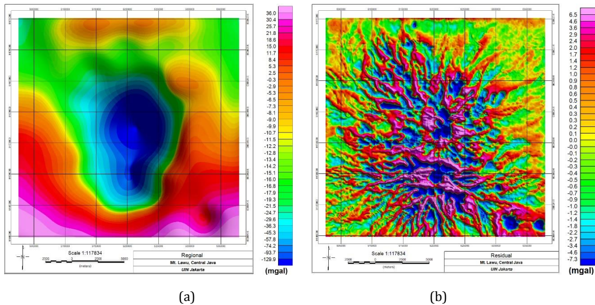
Figure 5. (a) Mountain Regional Map Lawu and (b) Mountain Residual Map Lawu
