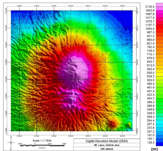
Figure 4. Digital Elevation Model (DEM) Map
