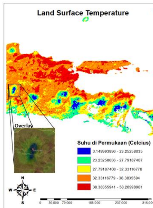
Figure 2. Land Surface Temperature (LST) Map
