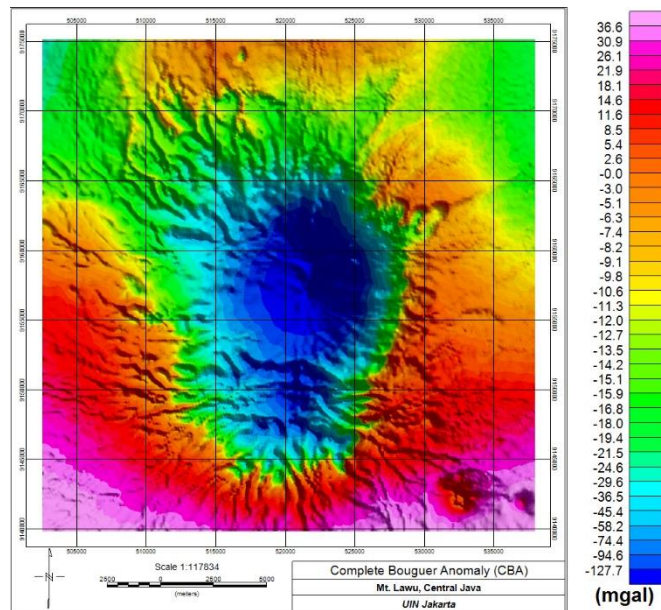
Figure 3. Complete Bouguer Anomaly (CBA) Map
