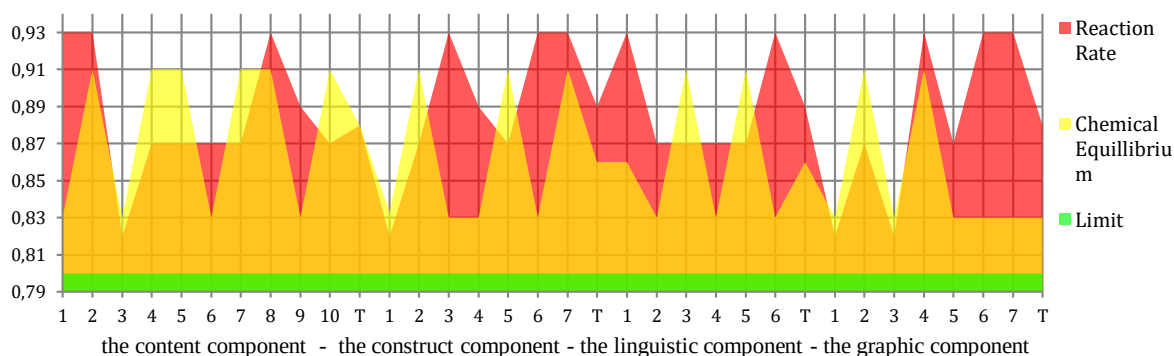
Figure 6. Comparison of the validity limit (green) with the validity of reaction rate (red)
