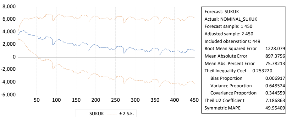
Figure 2. Forecast ARDL
