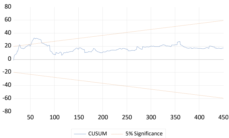
Figure 1. CUSUM
